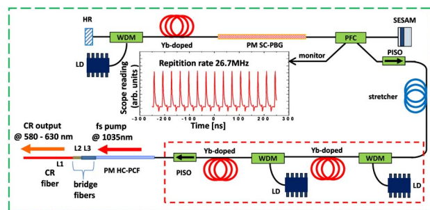
Fig. 1. (Color online) Layout of the all-fiber Cherenkov source. HR, high-reflectivity pigtailed mirror; WDM, 980/1030 wavelength division multiplexer; LD, single-mode pumping diode at 974 nm; PM SC-PBG, polarization-maintaining all-solid photonic bandgap fiber; SESAM, semiconductor saturable absorber mirror; PISO, polarization-maintaining isolator; PFC, 80/20 polarization filter coupler; HC-PCF, laser pulse compressor hollow-core PCF; CR fiber, highly nonlinear fiber for CR generation. (Inset) Oscilloscope reading of the mode-locked pulse train.
