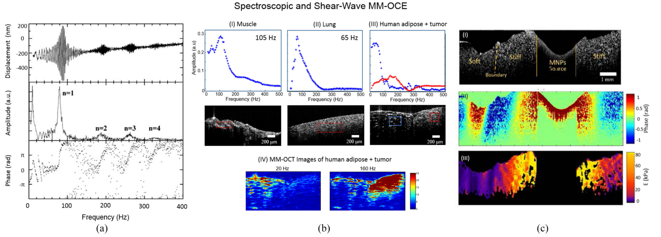
Fig. 4. Spectroscopic and shear-wave MM-OCE. (a, b) Spectroscopic MM-OCE is an alternative way of determining the resonant/natural frequency. (a) Excited by a chirp waveform, a cylindrical agarose sample exhibits (top) a frequency-dependent displacement, where (middle) the computed amplitude reveals the longitudinal resonance modes n = 1, 2, 3, 4 , and (bottom) the phase shift from 0 to \pi across each resonance mode agrees with theoretical expectation [72]. (b) Spectroscopic MM-OCE with a two-dimensional imaging scheme was applied to probe the biomechanical properties of the sample both spatially and temporally, where the mechanical spectral response can be revealed in both (I, II) homogenous rat muscle and lung tissues and (III, IV) more heterogeneous tissues such as at the tumor-adipose margin in human breast tissue. (IV) A stronger MM-OCT signal is seen at lower excitation frequencies for softer tissue and at higher frequencies for the stiffer areas (tumor) [75]. (c) Shear-wave MM-OCE shown in (I) a heterogeneous agarose sample where a clear boundary between stiff and soft regions can be seen. (II) The wave propagation can be visualized and further used for (III) Young's moduli quantification and mapping [74].
