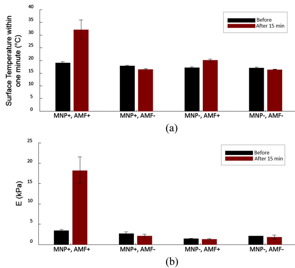
Fig. 6. Surface temperature and Young's modulus results of the four groups (black) before and (dark red) after 15 min of treatment. (a) Surface temperature measured within a 1-min time interval ( T_{1-\text{min}} ) at six different locations on each sample. A significant temperature rise is observed only in the MNP+, AMF+ case, indicating the effectiveness of the magnetic hyperthermia. (b) Validating Young's moduli were obtained from indentation testing. A significant increase in stiffness occurred only in the MNP+, AMF+ tissue.
