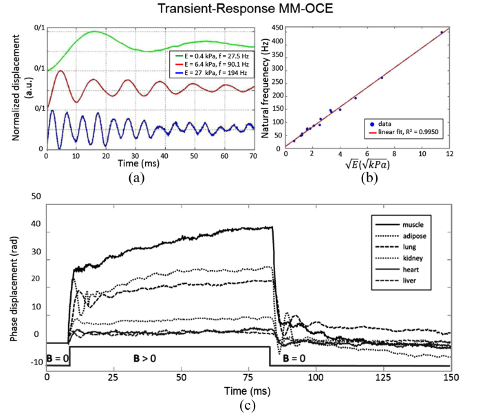
Fig. 3. Transient-response MM-OCE detecting the natural frequency of a material. (a) A correlation between the natural frequency and stiffness can be seen. This correlation is quantitatively shown in (b), where a linear dependence between the natural frequency and square root of the Young's modulus can be observed [71]. (c) Results show how the natural frequency can be used to characterize the viscoelastic behavior of different ex vivo rabbit tissues [73].
