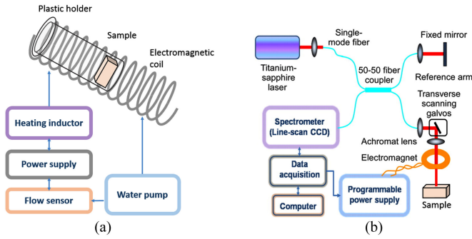
Fig. 5. Schematic of (a) the magnetic hyperthermia and (b) MM-OCE systems. The MM-OCE setup schematic is adapted from [11].
