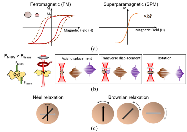
Fig. 1. Classification and properties of MNPs. (a) Typical \vec{M} - \vec{H} curve of (left) ferromagnetic (FM) and (right) superparamagnetic (SPM) particles, where the hysteresis loop and remnant magnetization ( \vec{M}_r ) is present in the FM particles. (b) Schematic of the sample arm in a MM-OCT setup where (left) MNP-laden tissue is located beneath the magnetic coil. (Left) The magnetic force on the tissue and (right) different forms of magnetomotion are illustrated in relation to the OCT imaging beam (adapted from [11], [21]). (c) Heating mechanisms of SPM nanoparticles, where (left) Néel rotation describes the internal rotation of the magnetic moment (shown as arrows), and (right) Brownian rotation is the rotation of the entire particle.
