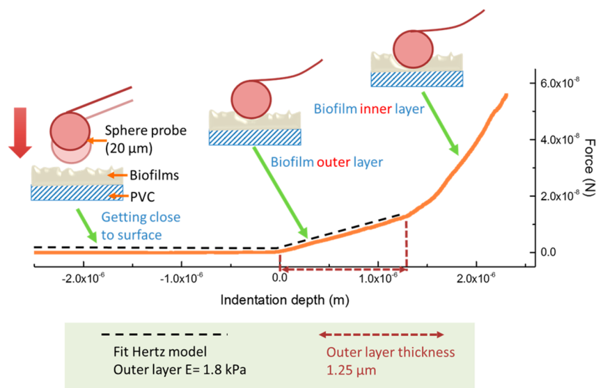
Figure 2. Indentation test principle. A sphere probe with the diameter of 20\ \mu\text{m} was used in the indentation measurement. When the probe was indented into the biofilm surface, the deflection of the probe cantilever was monitored, and the applied force was calculated with the measured vertical deflection and the spring constant of the cantilever. The force as a function of indentation depth was then plotted, and the biofilm outer layer Young's modulus and thickness was determined accordingly.
