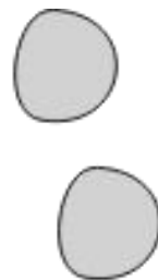
not simply connected
