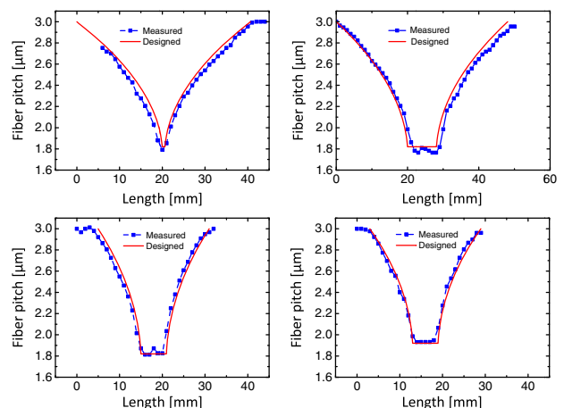
Fig. 7. Examples of different designs (solid line) and their practical realizations (dots) for PCF tapers.
