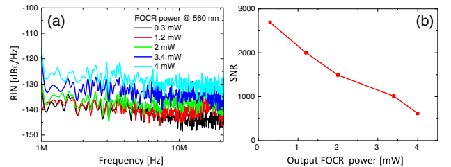
Fig. 14. Noise measurements of the FOCR pulses dependent on the output power. (a) Noise spectra of the FOCR pulses versus output power at FOCR wavelength of 560 nm. (b) The SNR of FOCR dependent on the output power.
