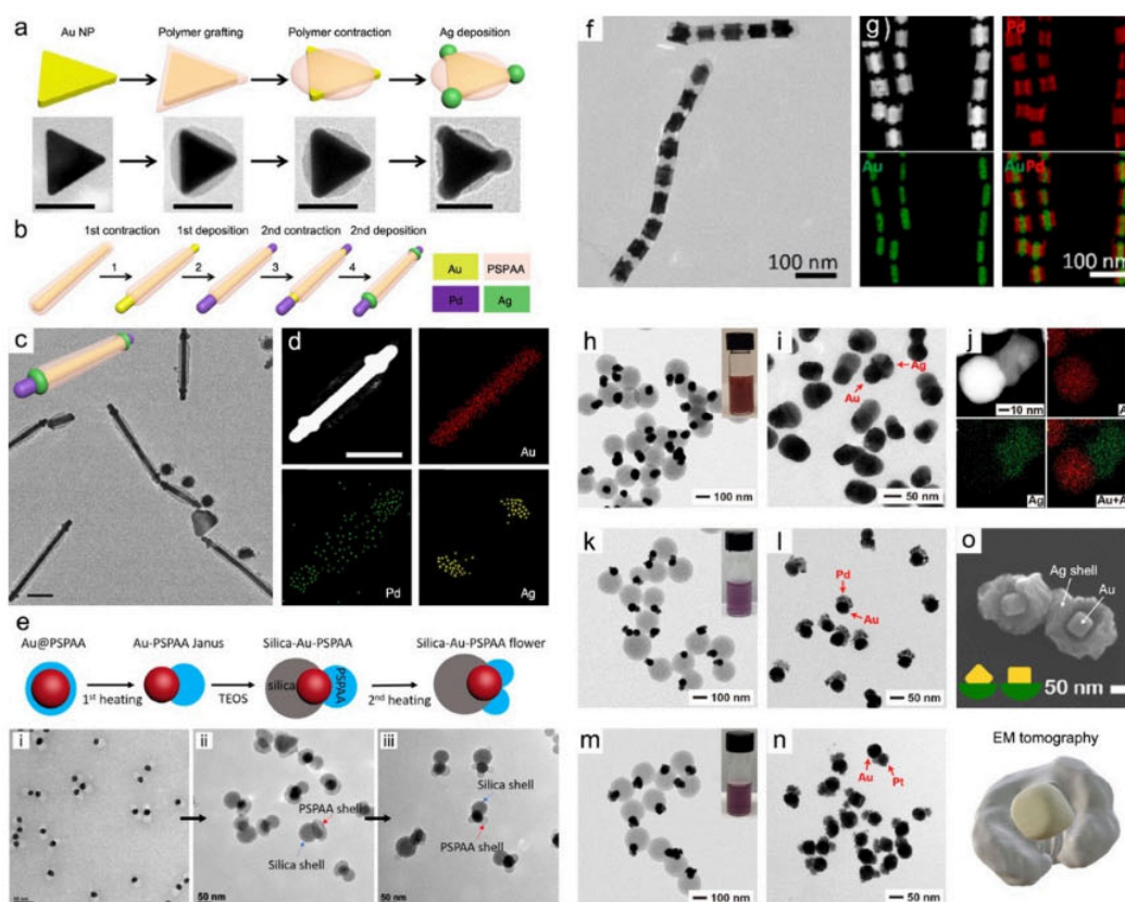
Figure 13. Patchy Au NPs as templates for overgrowth. (a) Schematics and TEM images illustrating the overgrowth of Ag on PS- b -PAA patchy Au nanoprisms. (b–d) Schematics (b), TEM image (c), and energy dispersive X-ray (EDX) mapping (d) of patchy Au NRs subsequently deposited with Pd and Ag via multi-step overgrowth. (e) Schematics and TEM images of silica-overgrown Janus Au NPs. (f) TEM and (g) EDX mapping of chain-like assemblies of patchy Au NRs after Pd-overgrowth. (h) TEM images of Au–PS Janus NPs after Ag overgrowth. (i) TEM and (j) EDX mapping of Au–Ag Janus NPs after selective removal of PS patch. (k,l) TEM images of Pd-overgrown Au–PS Janus NPs before (k) and after (l) selective removal of PS patch. (m,n) TEM images of Pt-overgrown Au–PS Janus NPs before (m) and after (n) selective removal of PS patch. The top-right insets in (h), (k), and (m) show Au–PS Janus NP solutions after metal overgrowth. (o) SEM image (top) and EM tomography (bottom) of Au–Ag bowl-like NPs after selective removal of PS- b -PAA patch. Scale bars: (a) 50 nm and (c,d) 100 nm. (a–d) Reproduced with permission from ref. [46]. Copyright 2018, Springer Nature. (e) Reproduced with permission from ref. [47]. Copyright 2019, American Chemical Society. (f,g) Reproduced with permission from
