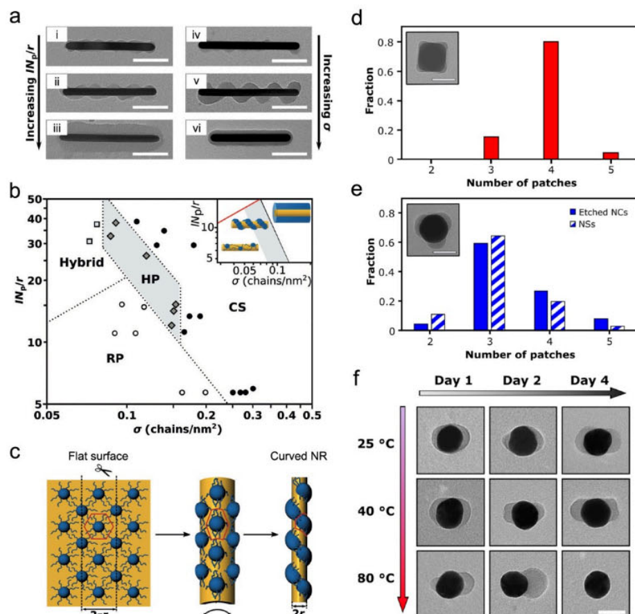
Figure 2. Solvent-mediated segregation of homopolymer ligands on anisotropically shaped Au NPs. (a) Representative TEM images of patchy Au NRs synthesized under varying lN/r and \sigma . (b) Experimental diagram of polymer pattern states as a function of lN/r and \sigma for the Au NRs. (c) Schematic illustrating the formation of the helicoidal patches on NRs. (d,e) Histograms of patchy Au NCs (d), as well as etched Au NCs and Au NSs (e) with different n . (f) Representative TEM images of patchy Au NSs after thermal treatment at different temperatures for varying durations. Scale bars: (a) 100 nm, (d,e) 50 nm, and (f) 40 nm. (a–c) Reproduced with permission from ref. [28]. Copyright 2019, Wiley-VCH. (d,e) Reproduced with permission from ref. [29]. Copyright 2017, American Chemical Society. (f) Reproduced with permission from ref. [33]. Copyright 2020, American Chemical Society.
