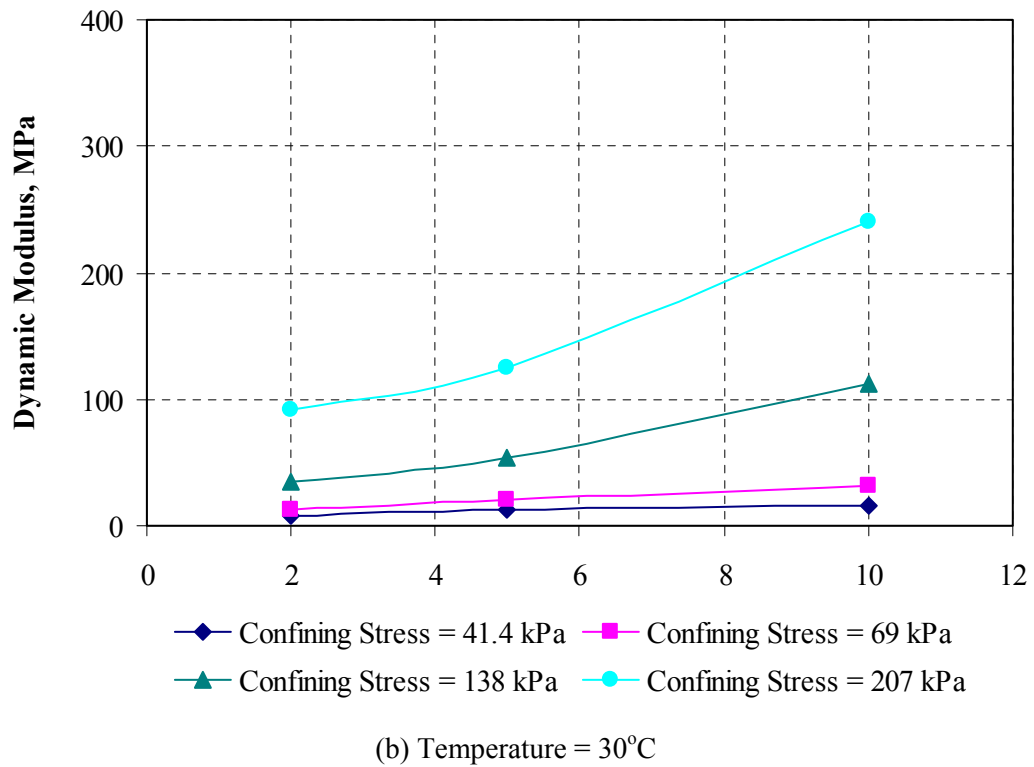
FIGURE 8.20 Effect of Loading Frequency on Dynamic Modulus for SE-14.
