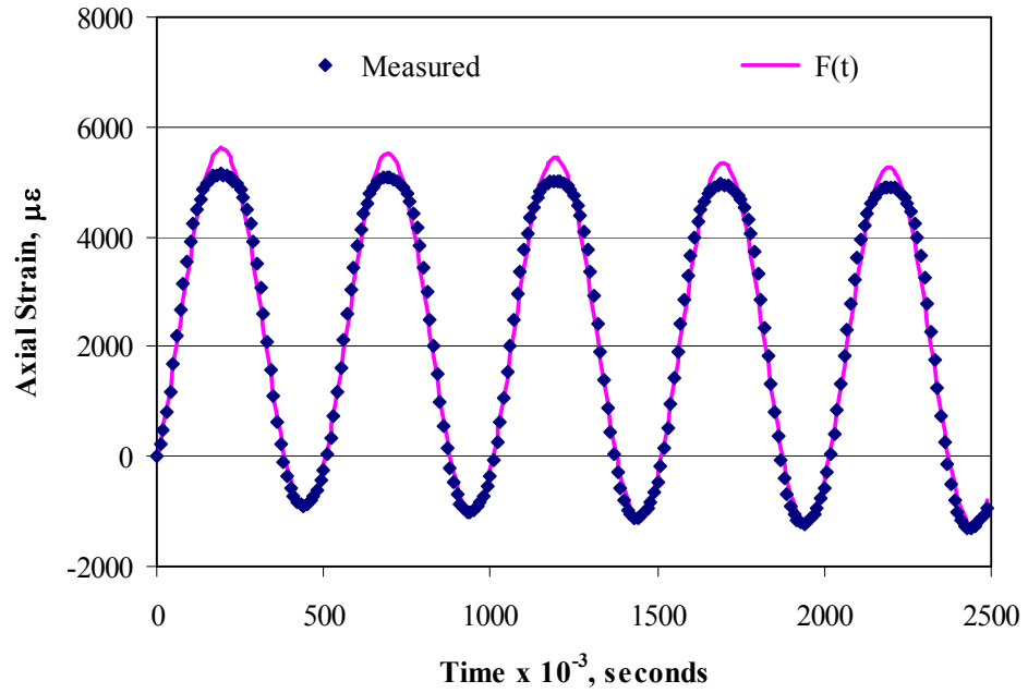
FIGURE 8.1b Variation of Strain with Time for Typical Test Results of Oil Sand Material.
