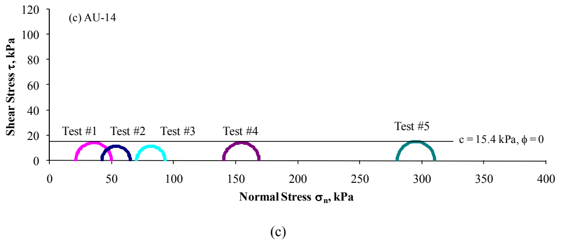
FIGURE 5.6 Mohr Circles for Oil Sand Samples at 30°C.
