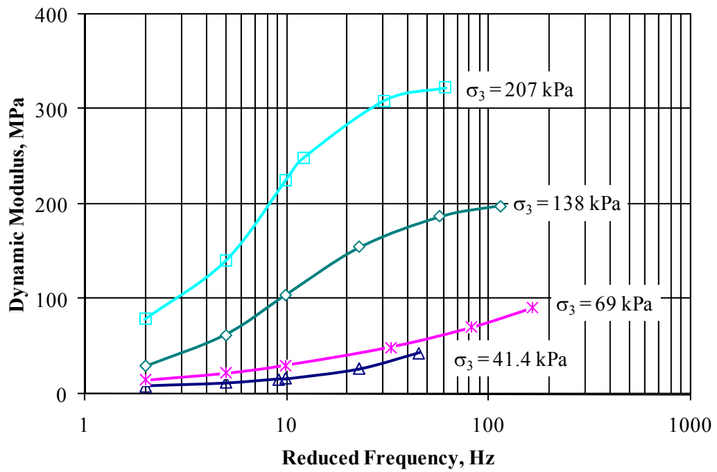
FIGURE 8.29 Master Curves for SE-14 Oil Sand Sample.
