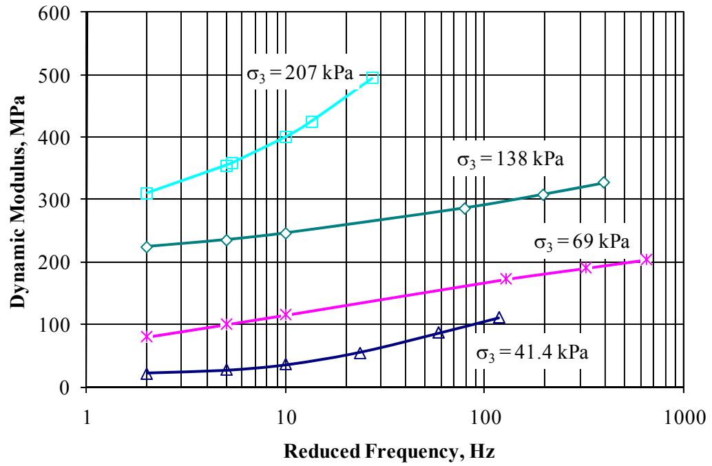
FIGURE 8.28 Master Curves for SE-09 Oil Sand Sample.
