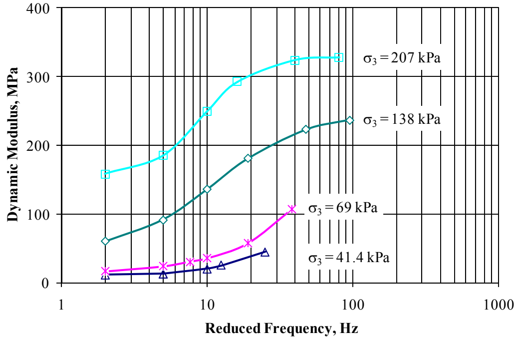
FIGURE 8.30 Master Curves for AU-14 Oil Sand Sample.
