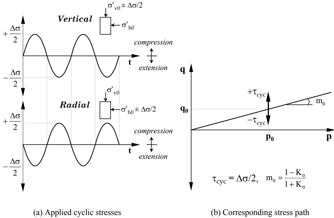
FIGURE 3.9 Pure Shear Loading Applied on the Specimen.
