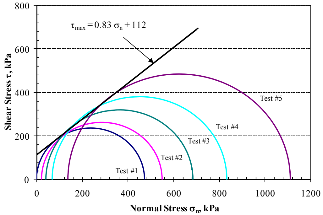
FIGURE 5.3 Mohr Circles and Failure Envelope for CAT A-6 Soil at w_{opt} = 14.3\% .
