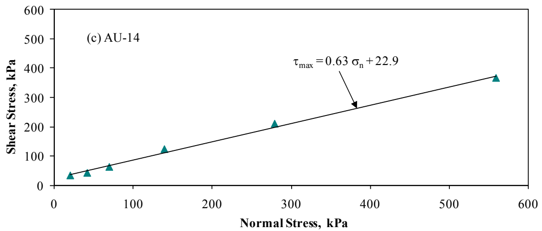
FIGURE 5.7 Mohr-Coulomb Failure Envelopes for Oil Sand Samples at 20°C.
