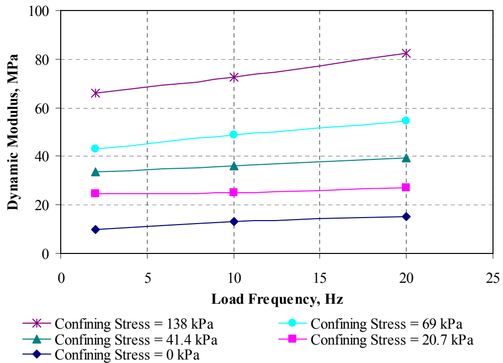
FIGURE 8.10 Effect of Loading Frequency on Dynamic Modulus at w = 17.3\% .
