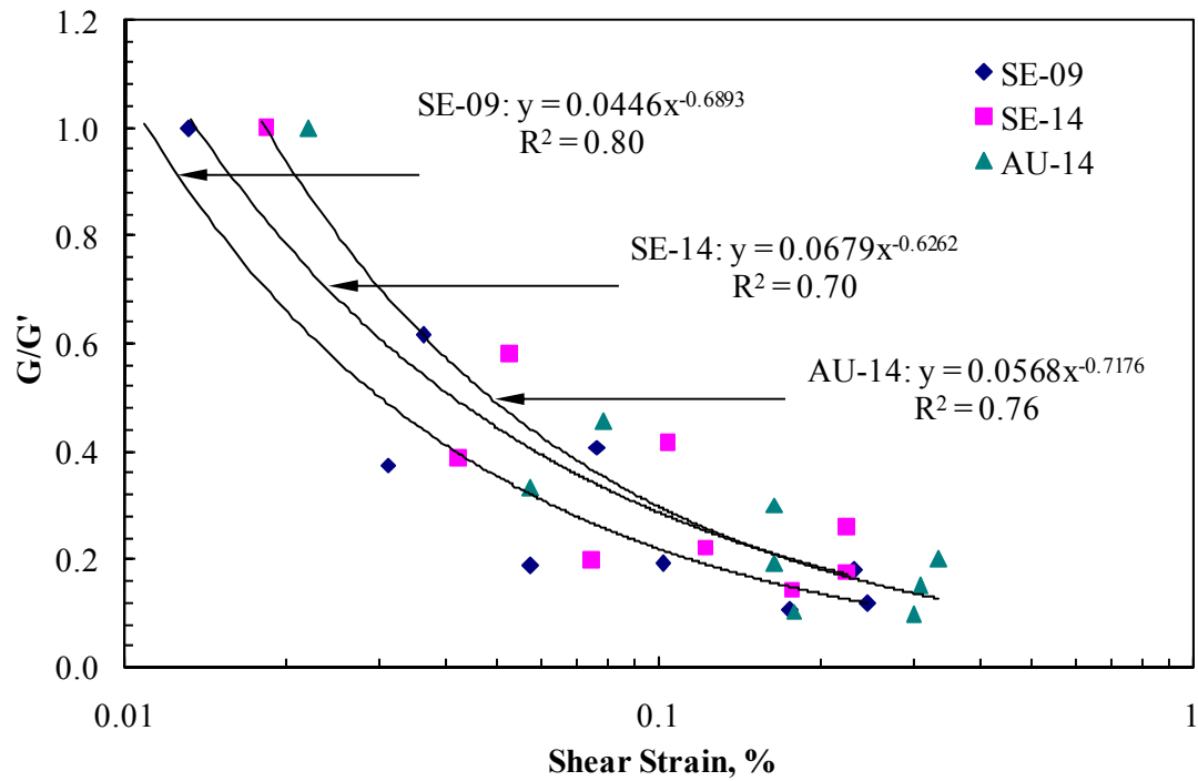
FIGURE 7.11 Normalized Shear Moduli of Oil Sand Samples against Shear Strain at 10Hz and 30°C.
