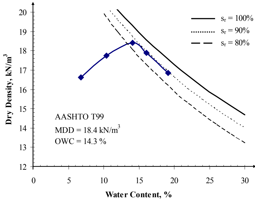
FIGURE 3.2 Standard Proctor Moisture-Density Characteristics of Fine-Grained Soil
