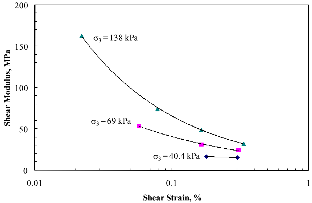
FIGURE 7.8b Variation of Shear Modulus with Shear Strain: AU-14 at 10Hz and 30°C.
