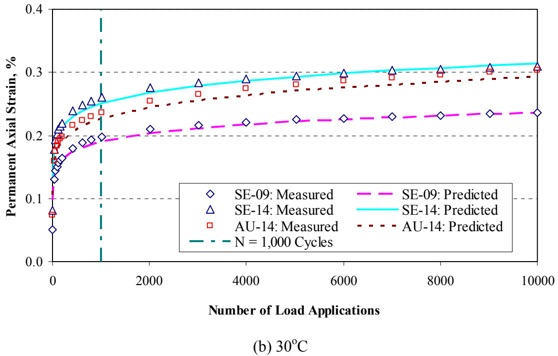
FIGURE 6.10 Permanent Strain Model Predictions for Additional Test Specimens: (a) Temperature = 20°C and (b) Temperature = 30°C.
