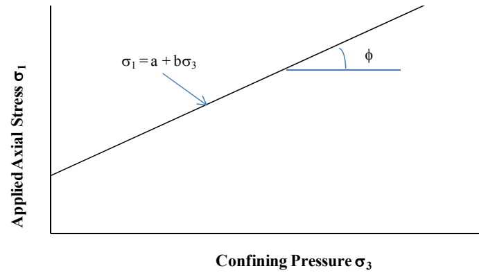
FIGURE 3.7 Relationship between Axial Stress and Confining Pressure.
