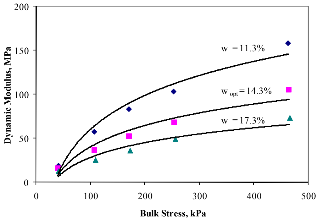
FIGURE 8.11 Variation of Dynamic Modulus of CAT A-6 Soil with Bulk Stress at three Moisture States.
