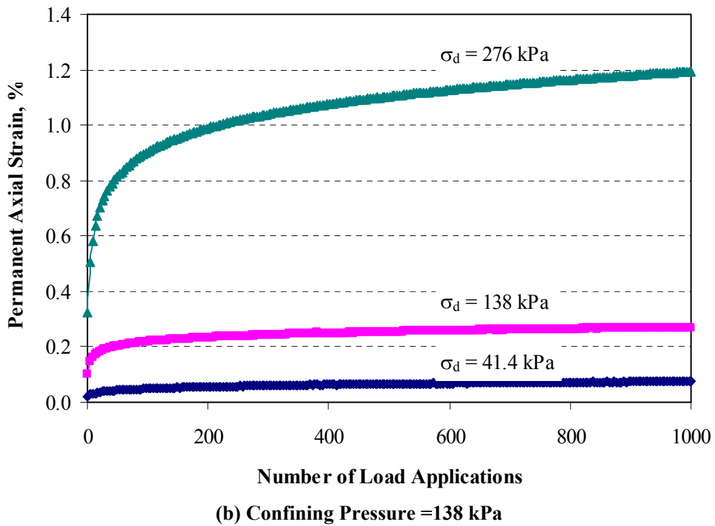
FIGURE 6.5 Effect of Deviator Stress on Permanent Strain Accumulation in AU-14 Sample: (a) Confining Pressure = 41.4 kPa, (b) Confining Pressure = 138 kPa and (c) Confining Pressure = 276 kPa.
