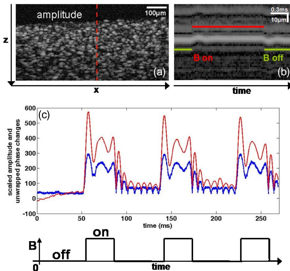
Fig. (8). Scatterer response upon step-wise modulation of a magnetic field. (a) Two-dimensional (x-z) cross-sectional (B-mode) amplitude OCT image of a silicone sample containing MNPs and TiO 2 optical scatterers. The dashed line indicates the location in sample where M-mode imaging is performed with MM-OCE. (b) M-mode amplitude OCT image of a region of scatterers acquired while the magnetic field is applied step-wise. (c) Average time-dependent scatterer changes along one axial position, illustrating both the changes in phase (red) and changes in amplitude (blue) as the magnetic field is applied step-wise, relative to an idle state with zero magnetic field. Figure reproduced with permission from [100]. Copyright, Optical Society of America, 2009. (For interpretation of the references to color in this figure legend, the reader is referred to the web version of this paper).
